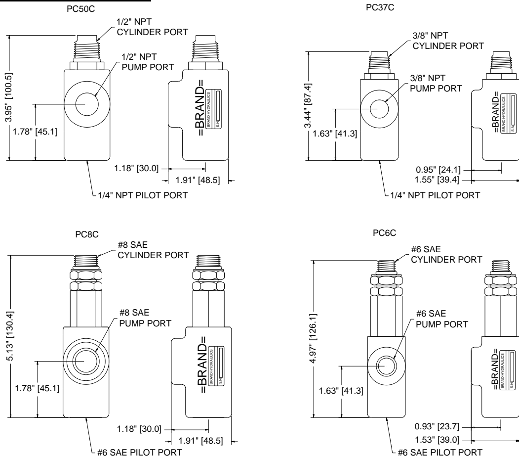
Figure 1: Dimensional Data for PC style valves in inches & [millimeters].
