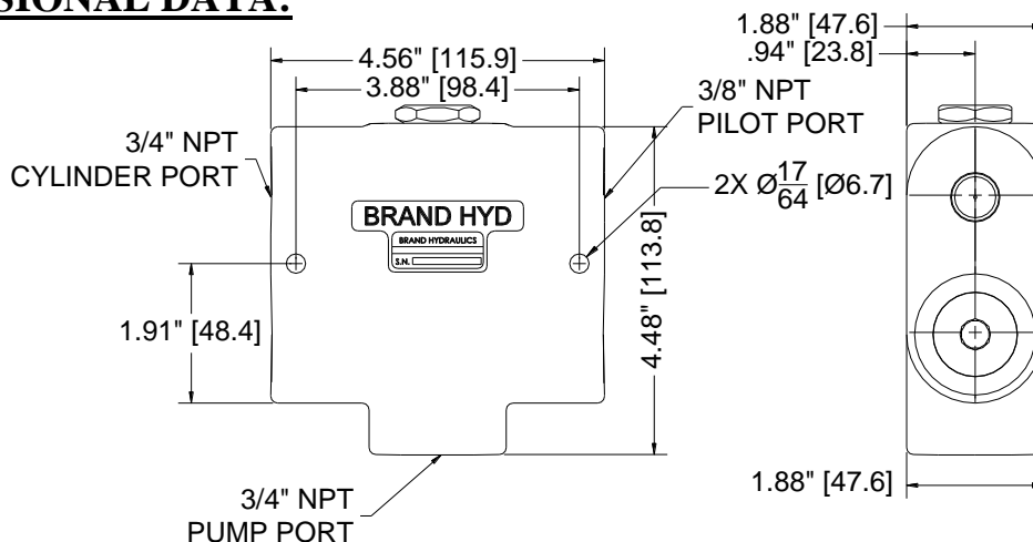
Figure 1: Dimensional Data for Pilot Operated Check valve in inches & [millimeters].
